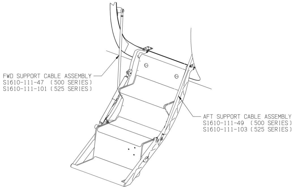
Figure 1 Support Cable Assemblies
