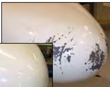
Above: Unretouched photo of eroded radome.
