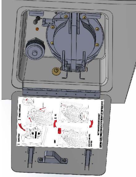
525/525A: Large Waste Valve Installation
