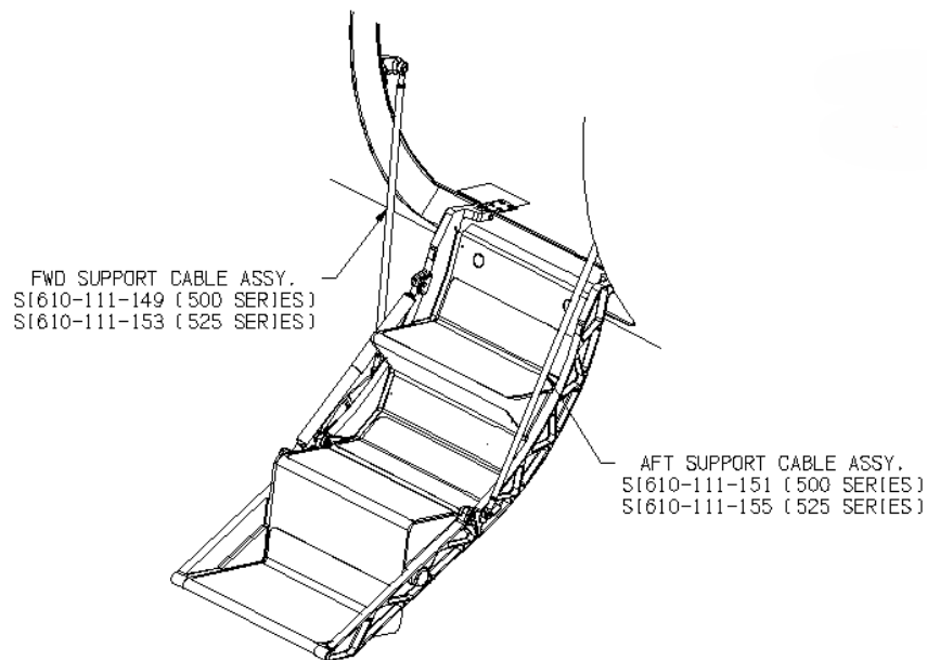
Figure 1 Support Cable Assemblies
