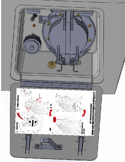
525/525A: Large Waste Valve Installation
