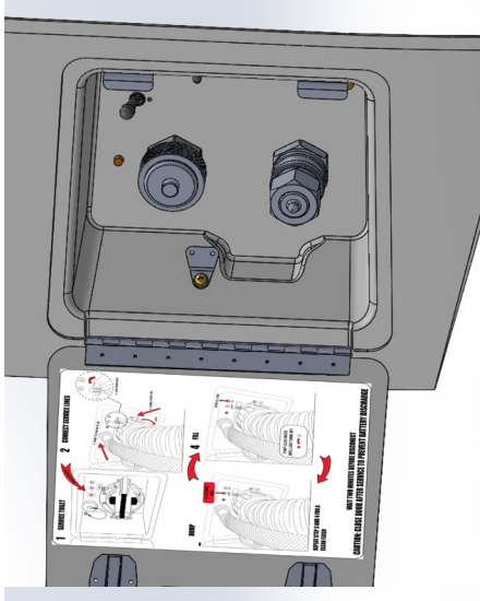
525/525A: Small Waste Valve Installation
